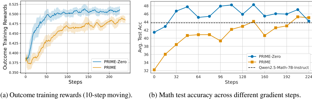
Figure 12: “Zero” RL from Qwen2.5-Math-7B. RL from the base model converges way faster than the SFT model, surpassing the instruct version within 32 steps.
