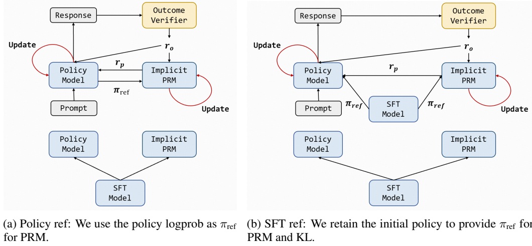
Figure 7: Comparison of different reference policy implementations. One uses the running policy’s old logprobs as reference (policy ref) while the other uses the initial SFT model as the reference model (SFT ref).
