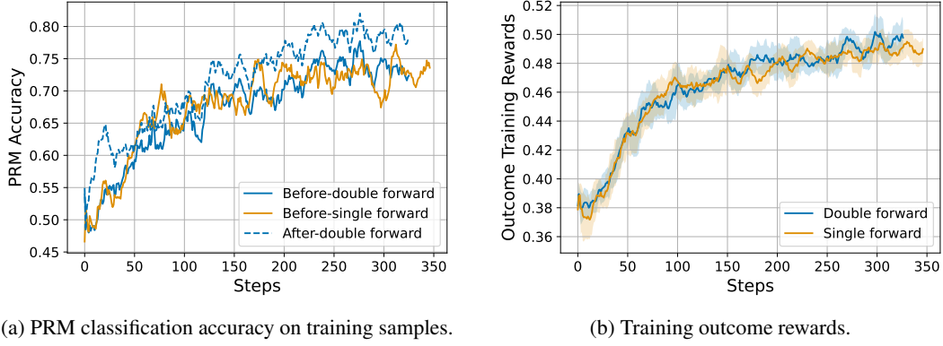
Figure 9: Single and double forward. While double forward methods obtain higher accuracy after online update, the two variants achieve similar rewards during training.
